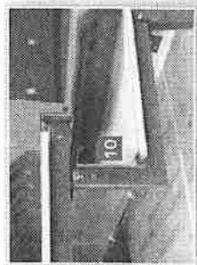
Nosebeam Splice web-bolt pattern
